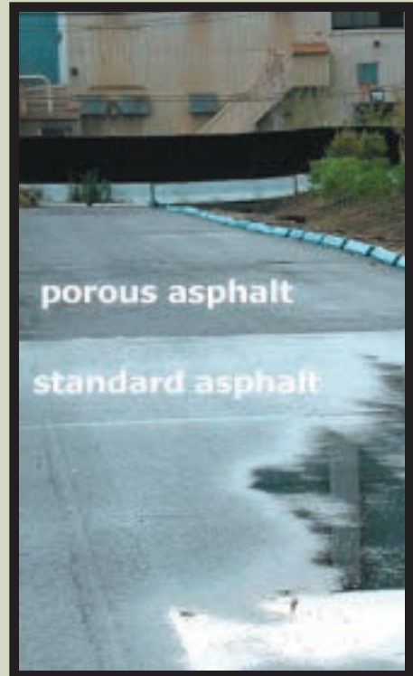
Figure 9 – The porous and standard sections of Ford Motor Co.'s lot.
