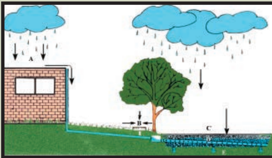
Figure 4 – Roof leaders can be connected directly to the subsurface infiltration bed.
